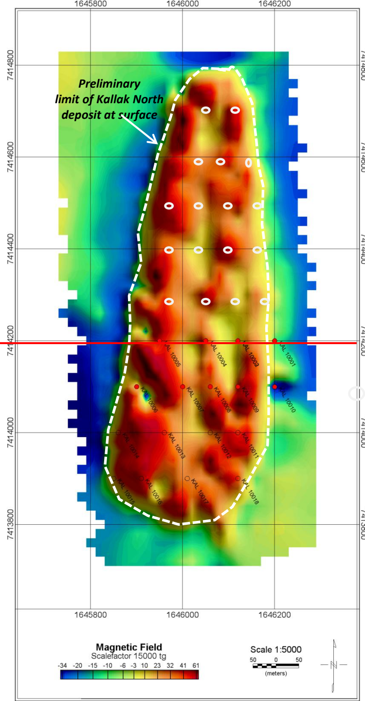
Fig 1 BEOWULF MINING plc KALLAK IRON ORE PROJECT Jokkmokk, N. Sweden Diamond drilling program 2010 Ground magnetic map Diamond drillholes completed and planned
